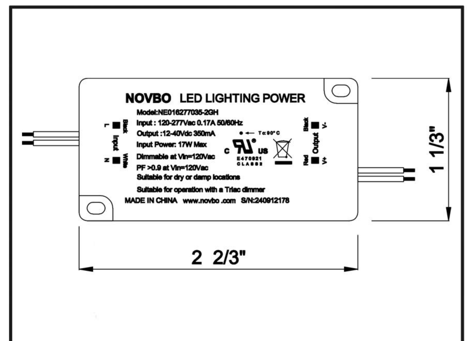
LED DRIVER DIAGRAM
