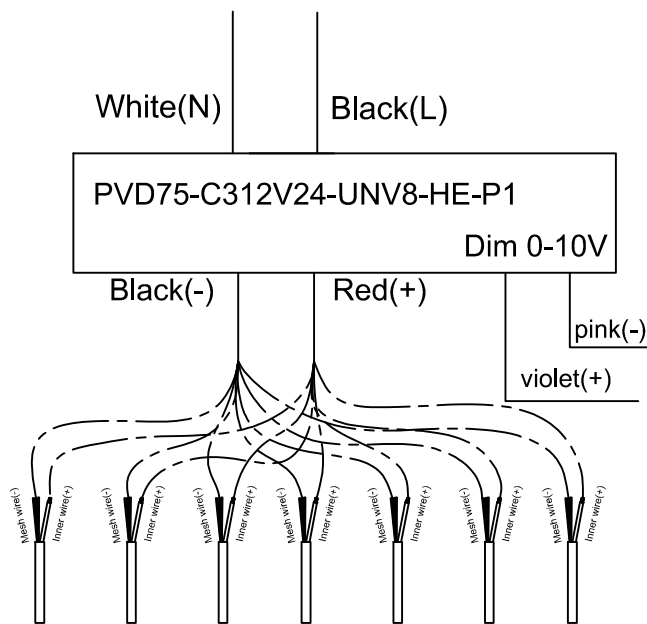
FACTORY CONNECTIONS (+) INNER CONDUCTOR | OUTER MESH (-)
